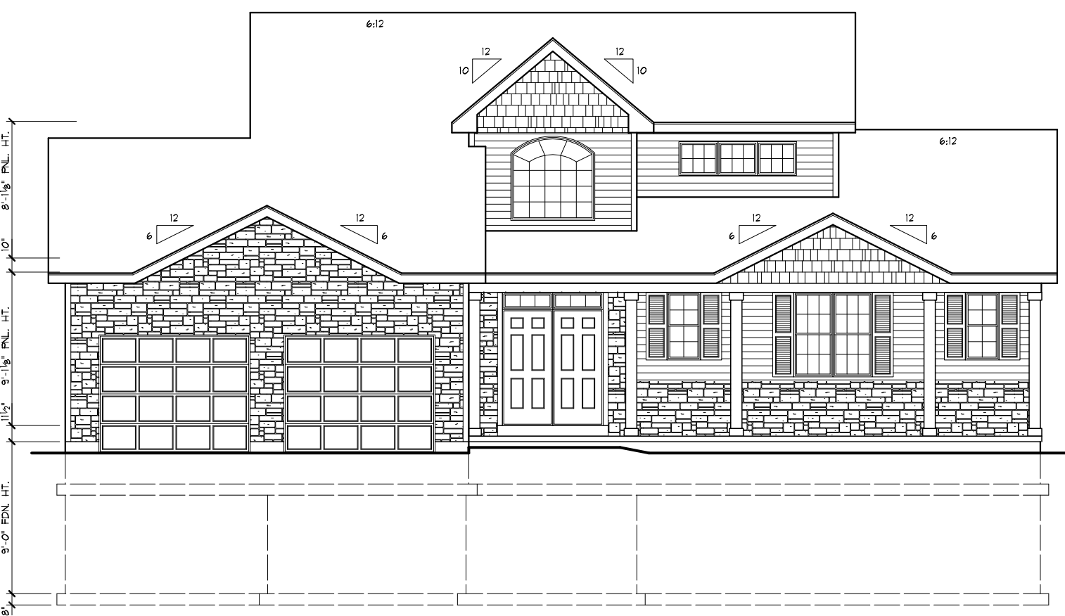
FRONT ELEVATION SCALE: 1/8"=1'-0" ON 11X17 1/4"=1'-0" ON 24X36
